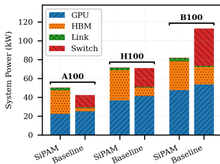
FIGURE 6. Power consumption breakdown of a rack-scale compute system across GPU–HBM generations, comparing the baseline configuration (72 GPUs per rack) and the SiPAM architecture (64 GPUs and a memory pool per rack).
