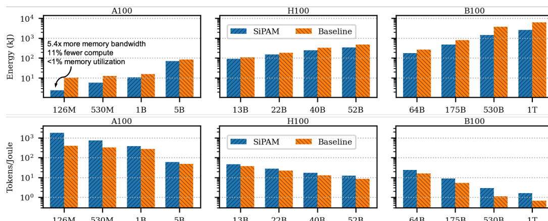
FIGURE 7. Comparison of inference energy consumption (top) and tokens per joule (bottom) across different workloads for SiPAM and baseline configurations.
