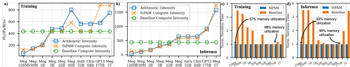
FIGURE 3. Arithmetic and compute intensity for training (a) and inference (b) of various Transformer-based workloads. Normalized iteration completion time for training (c) and inference (d). We label percentage memory utilization for two representative cases: memory bound workloads are provisioned with additional capacity to satisfy bandwidth demands, whereas compute bound workloads are allocated only the capacity required to fit the model.
