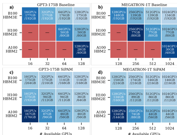
FIGURE 5. Heatmaps of iteration time for GPT-3 175B and Megatron-1T under varying cluster sizes and compute generations. (a) and (b) show baseline results; (c) and (d) show SiPAM results. Darker colors indicate higher iteration time. Red cells indicate no feasible parallelization strategy could fit the model. Text in cells show the number of actual GPUs used and memory utilization.
