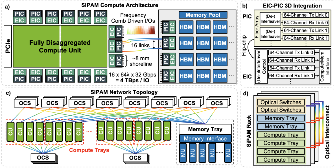
FIGURE 2. Schematic of (a) an example of the SiPAM compute architecture with frequency-comb-driven SiP I/Os embedded along the full periphery of a dual-die compute unit; (b) 3D integration of the EIC and the PIC for the SiP I/Os [4]; (c) the SiPAM network architecture which realizes a multi-dimensional all-to-all topology while adopting the intra-rack memory pooling model; and (d) the SiPAM intra-rack memory pooling structure for bounded latency.
