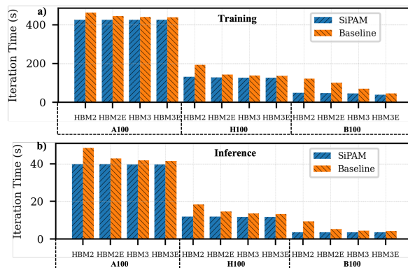
FIGURE 4. Iteration time across different combinations of compute and memory technology pairs for (a) training and (b) inference of GPT-3-175B.
