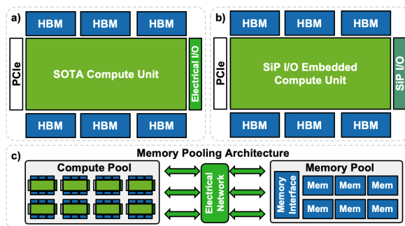
FIGURE 1. (a) Current compute architecture with on-package HBM stacks and high-speed electrical I/Os for networking. (b) CU with SiP I/Os replacing electrical interfaces. (c) Conventional memory pooling architecture connecting compute pools to memory pools using an electrically switched network.
